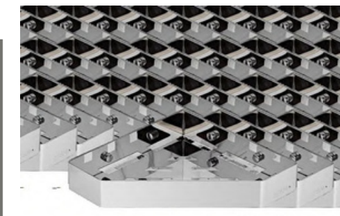
WT-514 Single Corner Basket Material:Stainless Steel 304 Size:290x60x210mm
