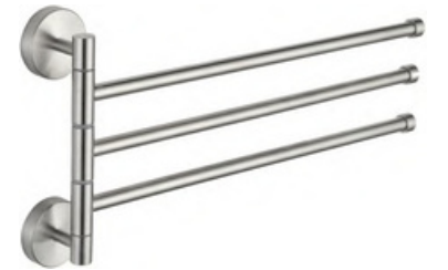
WT-3923 Swivel Towel Bar Material:Stainless Steel 304 Size:368x195x43mm
